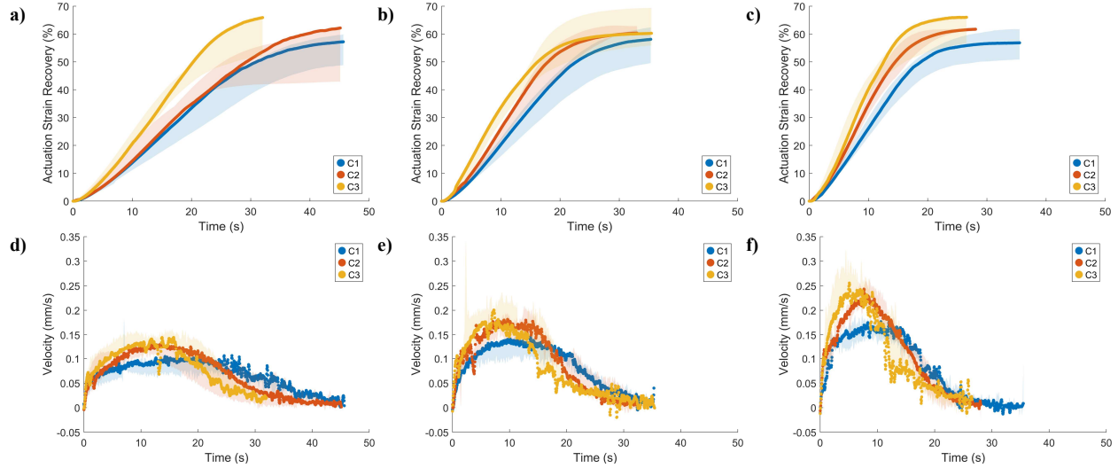
Figure 4. Median and shaded minimum-maximum %SR (top) and velocity (bottom) for each wire configuration at constant power levels of 4.2 W (left), 5.7 W (middle), and 7.0 W (right) ( n=3 for each curve).
