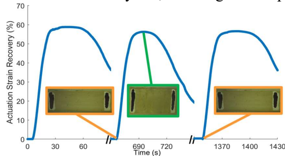
Figure 3. %SR vs. time for wire configuration C3 at a power level of 7.0 W for three heating-cooling actuation cycles, with images of the uncontracted and contracted sample taken before and during an actuation cycle, respectively.
