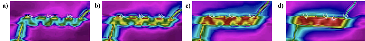
Figure 8. Thermal images of C1 sample at a) 5 s, b) 10 s, c) 20 s, and d) 45 s during heating at a constant power input of 7.0 W.
